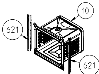
CAVITY ASSEMBLY EXPLODED VIEW
