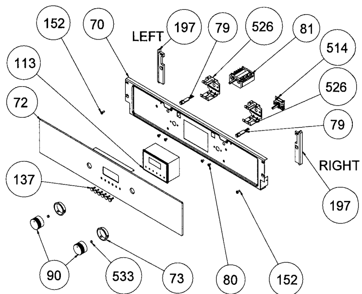
GLASS CONTROL PANEL ASSEMBLY ( OPTIONAL )
