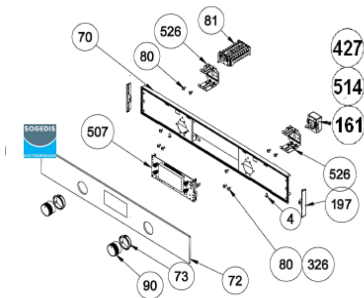
VISIO TOUCH GLASS CONTROL PANEL ASSEMBLY (OPTIONAL)
