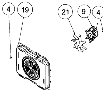
(FAN COVER/FAN IMPELLER ( 6 WINGS )/FAN MOTOR) (OPTIONAL)
